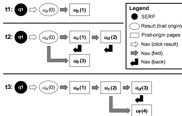
Figure 1. Web behavior graphs illustrating three trails.
